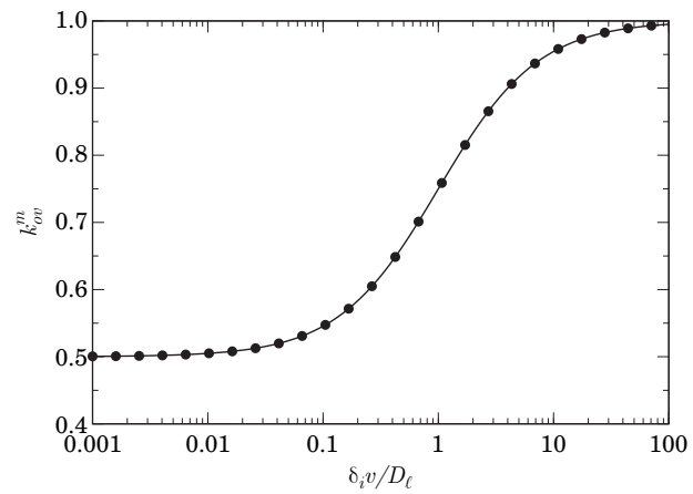
Fig. 2.25 Effective partition coefficient k_{0v} as a function of the dimensionless interface speed \delta_i v / D_\ell . For purposes of illustration, we have taken k_0^m = 0.5 . Copyright 2016 EPFL Press. This figure has been reproduced from Solidification , by J.A. Dantzig and M. Rappaz, for instructional purposes. For other uses, please contact the authors and the EPFL Press for written permission.
