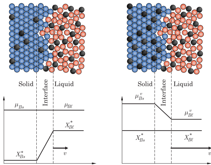
Fig. 2.23 Illustration of solute trapping for a diffuse solid-liquid interface. Notice that at higher velocity (right hand side) more solute atoms are “trapped” in the solid.
