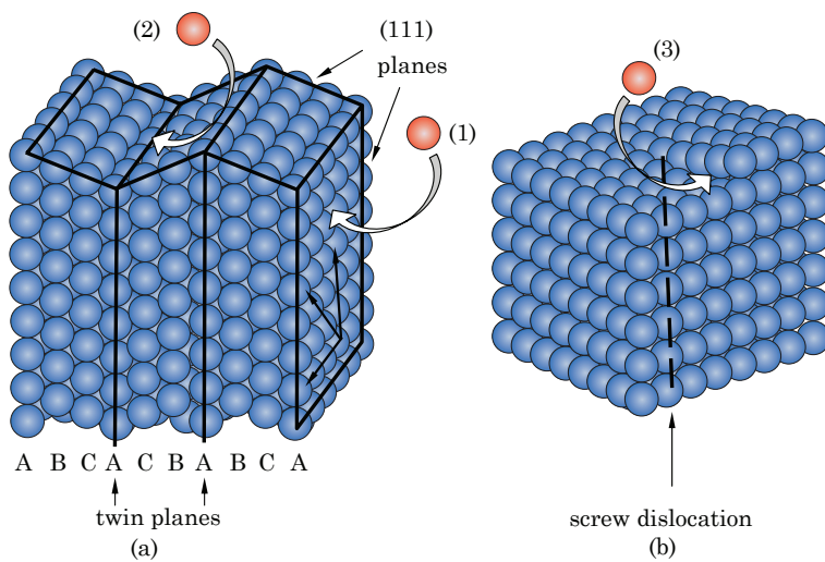
Fig. 2.22 (a) Illustration of secondary nucleation of an atom (1) on a (111) plane in a fcc lattice. In the same diagram, the double-twin mechanism of crystal growth is indicated for an atom (2). (b) Illustration of the screw dislocation growth mechanism in a simple cubic lattice with the attachment of atom (3) on the step. Copyright 2016 EPFL Press. This figure has been reproduced from Solidification , by J.A. Dantzig and M. Rappaz, for instructional purposes. For other uses, please contact the authors and the EPFL Press for written permission.
