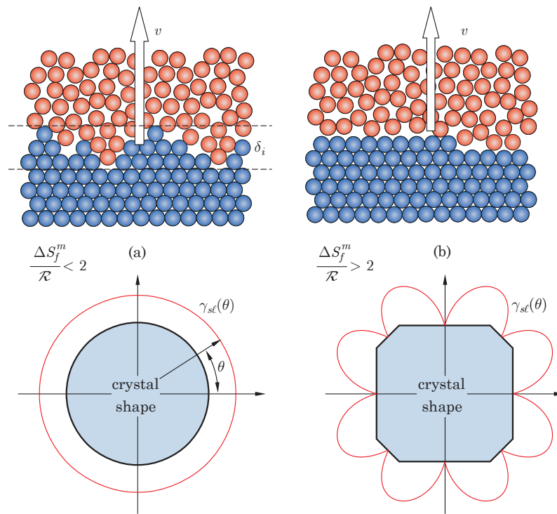
Fig. 2.21 Types of solid-liquid interfaces encountered in solidification (top): (a) diffuse interfaces typical of metals; (b) smooth interfaces typical of faceted materials. The associated \gamma -plots (red line) and equilibrium crystal shapes (blue shapes) are indicated at the bottom.
