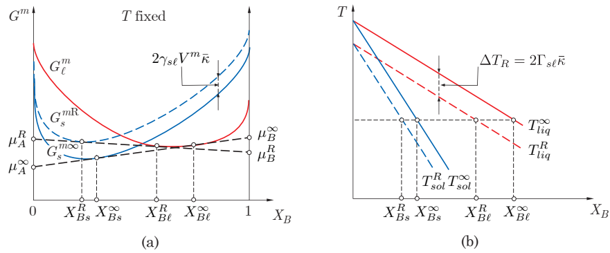
Fig. 2.20 Equilibrium of solid and liquid phases for a binary alloy including the curvature contribution. (a) shift in free energy curves, and (b) the shift in the liquidus and solidus curves on the equilibrium phase diagram.
