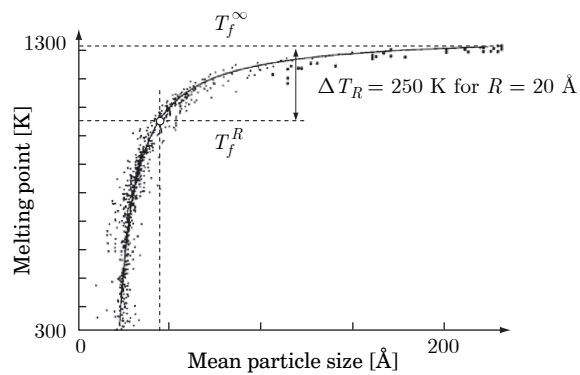
Fig. 2.19 Melting point of small gold particles as measured by electron diffraction techniques (courtesy of Ph. Buffat, EPFL [2]).
