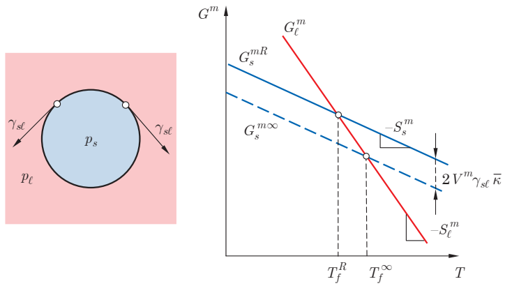
Fig. 2.18 Gibbs free energy for a solid sphere of radius R , and the condition of equilibrium with the liquid.
