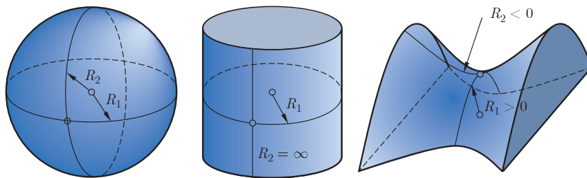
Fig. 2.17 Principal radii of curvature for a sphere, cylinder and saddle point. Copyright 2016 EPFL Press. This figure has been reproduced from Solidification , by J.A. Dantzig and M. Rappaz, for instructional purposes. For other uses, please contact the authors and the EPFL Press for written permission.
