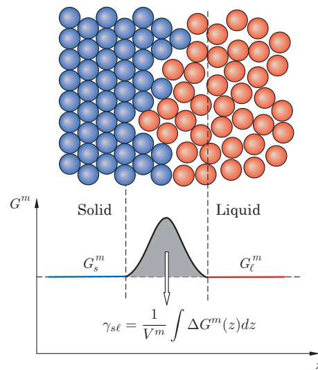
Fig. 2.16 Excess Gibbs free energy of atoms located within a diffuse solid-liquid interface and interfacial energy.
