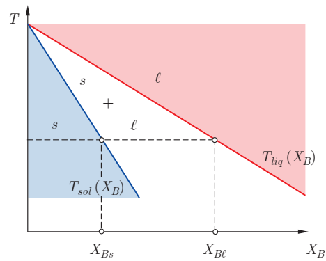
Fig. 2.14 Simple phase diagram showing the region where the two phases, solid and liquid, co-exist.
