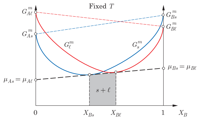
Fig. 2.13 Free energies of two phases, solid and liquid, as a function of the composition X_B showing the condition of equilibrium when they co-exist. Copyright 2016 EPFL Press. This figure has been reproduced from Solidification , by J.A. Dantzig and M. Rappaz, for instructional purposes. For other uses, please contact the authors and the EPFL Press for written permission.
