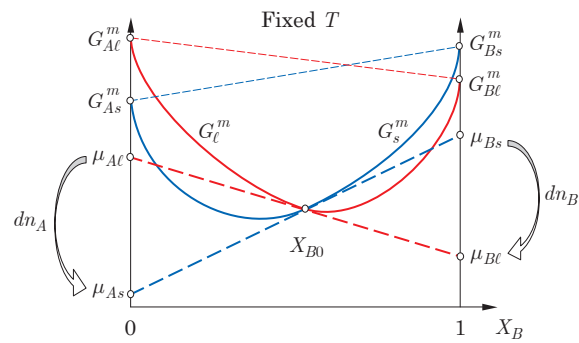
Fig. 2.12 Free energies of two phases, solid and liquid, as a function of the composition X_B and chemical potentials at the intersection of these two curves. Copyright 2016 EPFL Press. This figure has been reproduced from Solidification , by J.A. Dantzig and M. Rappaz, for instructional purposes. For other uses, please contact the authors and the EPFL Press for written permission.
