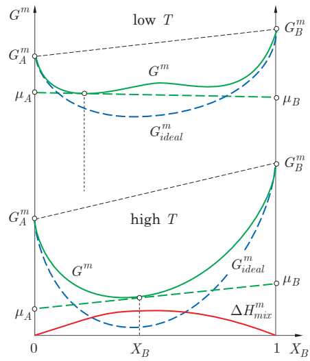
Fig. 2.11 Molar Gibbs free energy for a regular solution with \Omega^m > 0 at low and high temperatures. Copyright 2016 EPFL Press. This figure has been reproduced from Solidification , by J.A. Dantzig and M. Rappaz, for instructional purposes. For other uses, please contact the authors and the EPFL Press for written permission.
