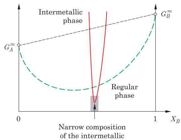
Fig. 2.10 Schematic of the Gibbs free energy of an intermetallic phase and intersecting a regular phase. Copyright 2016 EPFL Press. This figure has been reproduced from Solidification , by J.A. Dantzig and M. Rappaz, for instructional purposes. For other uses, please contact the authors and the EPFL Press for written permission.
