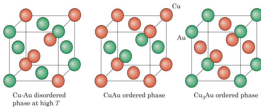
Fig. 2.9 Ordered phases in the Cu-Au system.
