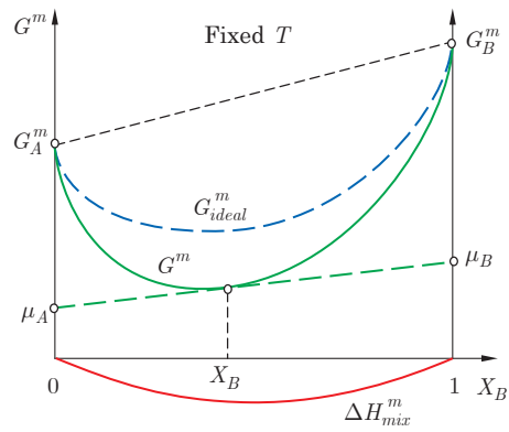
Fig. 2.8 Molar Gibbs free energy for a regular solution with \Omega^m < 0 at a fixed temperature. The chemical potentials are also indicated in this figure for a given composition.
