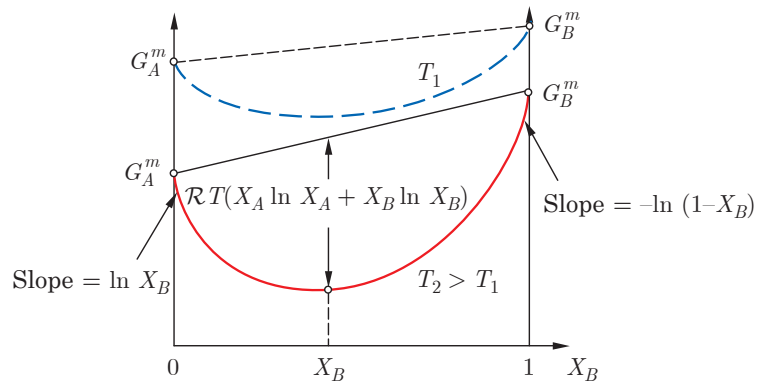
Fig. 2.7 Molar Gibbs free energy for an ideal solution at two temperatures T_1 < T_2 . Copyright 2016 EPFL Press. This figure has been reproduced from Solidification , by J.A. Dantzig and M. Rappaz, for instructional purposes. For other uses, please contact the authors and the EPFL Press for written permission.
