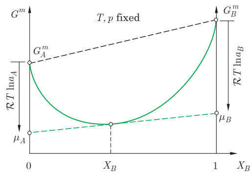
Fig. 2.6 Molar free energy of a binary solution as a function of the mole fraction of element B, showing the tangent construction to compute the chemical potentials \mu_A and \mu_B .
