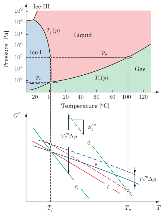
Fig. 2.3 Equilibrium phase diagram for water and schematic Gibbs free energies of the solid, liquid and gas phases at atmospheric pressure p_a (dashed curves) and at the triple point pressure p_t (solid lines). This figure is only schematic as V_g^m \approx 1250 V_\ell^m .
