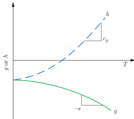
Fig. 2.1 Free energy and enthalpy as a function of temperature. Copyright 2016 EPFL Press. This figure has been reproduced from Solidification , by J.A. Dantzig and M. Rappaz, for instructional purposes. For other uses, please contact the authors and the EPFL Press for written permission.
