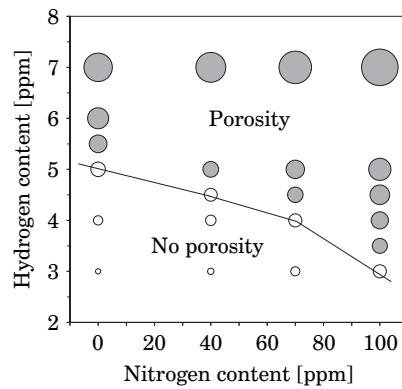
Fig. 12.25 The effect of gas content on porosity formation in AISI 8620 steel castings. The solid line separates castings expected to have porosity from those without it. Composition of the alloy (in wt%): 0.186 C, 0.83 Mn, 0.28 Si, 0.56 Cr, 0.55 Ni, 0.16 Mo, 0.015 P and 0.015 S. (From Sung et al. [21].)
