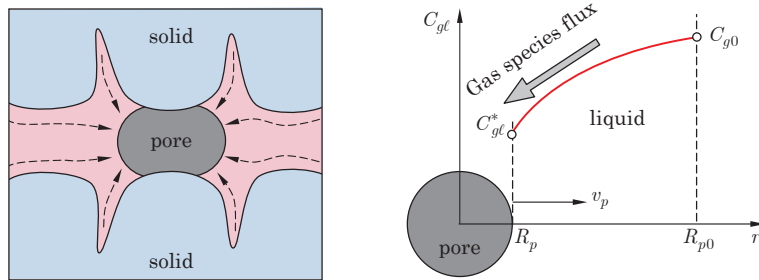
Fig. 12.18 Schematic views of (left) gas diffusion in between dendrite arms, and (right) composition profile in an ideal spherical geometry. Copyright 2016 EPFL Press. This figure has been reproduced from Solidification , by J.A. Dantzig and M. Rappaz, for instructional purposes. For other uses, please contact the authors and the EPFL Press for written permission.
