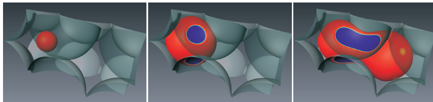
Fig. 12.17 Phase field simulation showing three stages of a small pore growing within a regular network of globular grains. The pore-solid interface is shown in blue, and the pore-liquid interface is in red. The solid grains are in grey and slightly transparent.[14]
