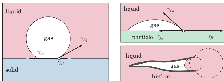
Fig. 12.14 The formation of a gas bubble at (left) the solid-liquid interface and (top right) the surface of a non-wetting particle. (bottom right) The growth of a gas pocket pre-existing in a bi-film of oxide.
