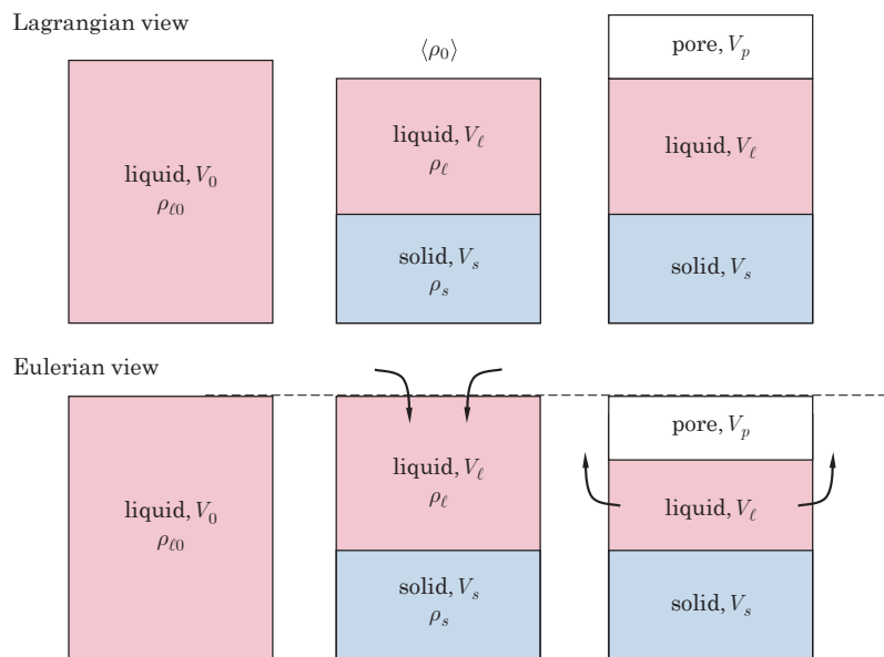
Fig. 12.13 The evolution of a closed volume in which solid and gas form from the liquid phase. In the Lagrangian view no mass is exchanged, whereas in the Eulerian view, mass enters or leaves to compensate volume changes.
