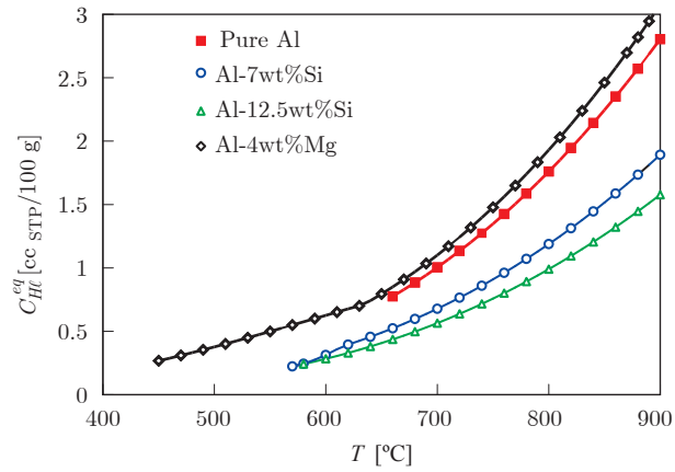
Fig. 12.11 The equilibrium composition of hydrogen in molten aluminum as a function of the temperature, showing the effect of Si and Mg additions. Copyright 2016 EPFL Press. This figure has been reproduced from Solidification , by J.A. Dantzig and M. Rappaz, for instructional purposes. For other uses, please contact the authors and the EPFL Press for written permission.
