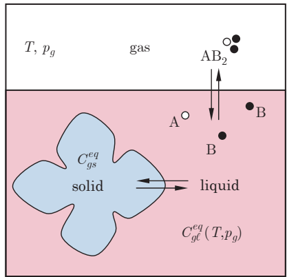
Fig. 12.10 The equilibrium between a gas, a liquid and a solid phase, with the schematic representation of a gas AB_2 and elements A and B in solution. Copyright 2016 EPFL Press. This figure has been reproduced from Solidification , by J.A. Dantzig and M. Rappaz, for instructional purposes. For other uses, please contact the authors and the EPFL Press for written permission.
