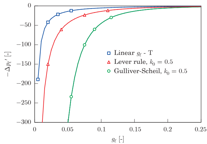
Fig. 12.8 The normalized pressure in the liquid as a function of g_\ell for an alloy of solidification interval \Delta T_0 with three microsegregation models g_\ell(T) . The pressure drop was normalized by the factor 5(S_V^\ell)^2 \beta \mu_\ell \Delta T_0 v_T / G .
