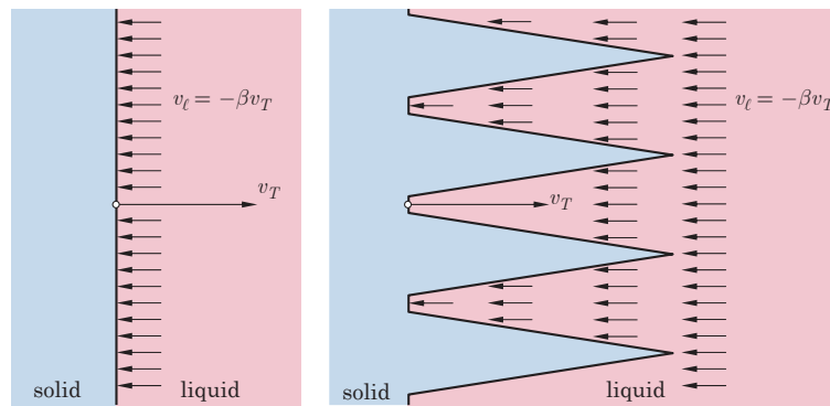
Fig. 12.7 Flow induced by shrinkage in a one-dimensional situation for two cases: (left) a planar front and (right) a schematic columnar growth in which g_s is a linear function of space.
