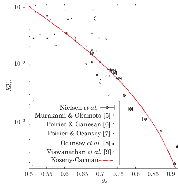
Fig. 12.6 The permeability K normalized by the square of the effective solid-liquid interface S_V^{s\ell} , measured by a variety of authors for various volume fractions of solid g_s . The dotted curve corresponds to the Carman-Kozeny relationship. (Courtesy of Ø. Nielsen, Sintef, Norway [15].)
