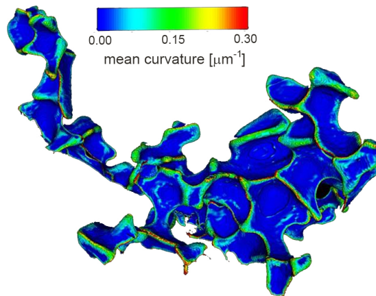
Fig. 12.4 A 3-D view of a shrinkage micropore in an inoculated Al-4.5wt%Cu alloy similar to that shown in Fig. 12.3. The reconstructed view obtained by X-ray microtomography has been colored according to the local mean curvature of the pore surface. (Courtesy of M. Felberbaum, EPFL).[8]
