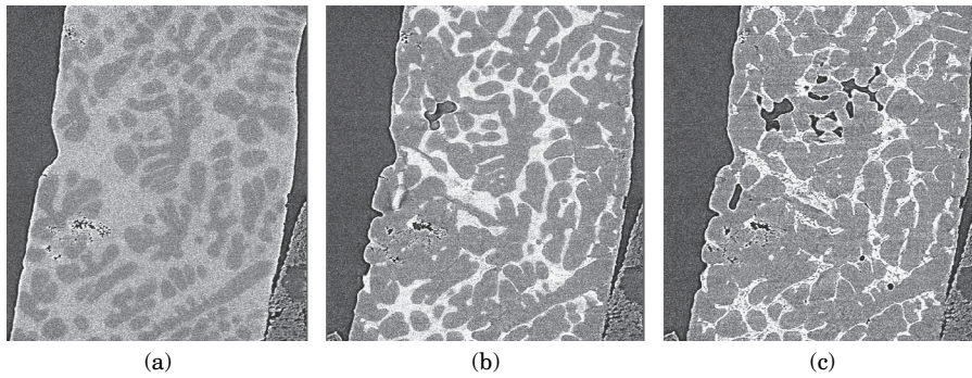
Fig. 12.3 A sequence of three X-ray tomography images from a longitudinal section, showing the formation of shrinkage porosity in a 1 mm diameter Al-10wt%Cu cylinder. (Courtesy of M. Suéry and L. Salvo, INPG, France.)
