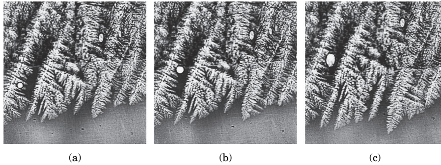
Fig. 12.2 A sequence of three X-ray radiographs showing the formation of gas porosity in a directionally solidified Al-30wt%Cu alloy, and its subsequent entrapment by the eutectic front. (Courtesy of R. Mathiesen, Sintef, Norway [13].) Copyright 2016 EPFL Press. This figure has been reproduced from Solidification , by J.A. Dantzig and M. Rappaz, for instructional purposes. For other uses, please contact the authors and the EPFL Press for written permission.
