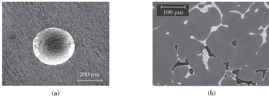
Fig. 12.1 (a) Gas porosity as observed by secondary electrons in scanning electron microscopy in an Al-10 wt%Cu alloy saturated with hydrogen in the liquid. (b) Shrinkage porosity observed by X-ray tomography in an Al-4.5 wt%Cu alloy. (Courtesy of M. Felberbaum.)
