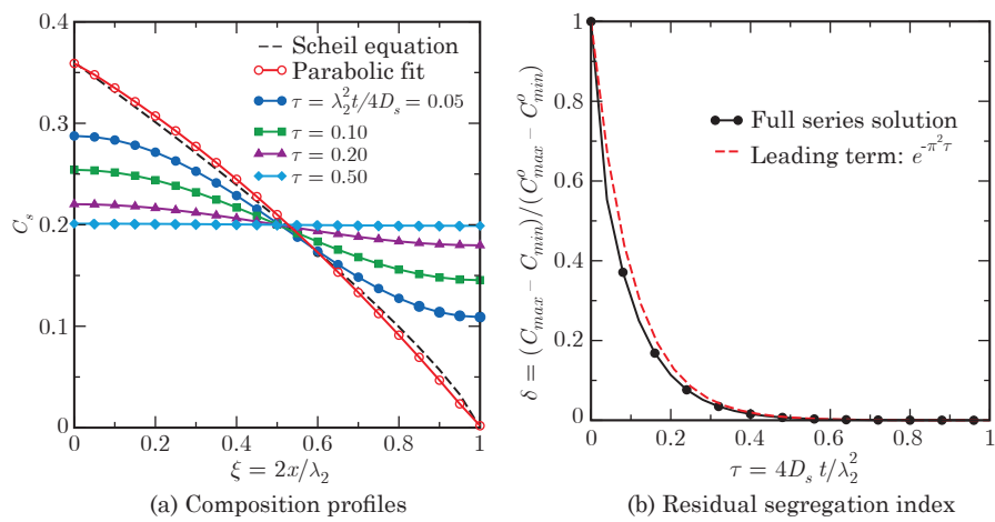
Fig. 10.11 The computed progress of the homogenization of a Cu-Ni alloy. (a) The evolution of the composition profile. (b) The residual segregation index, defined in Eq. (10.63).
