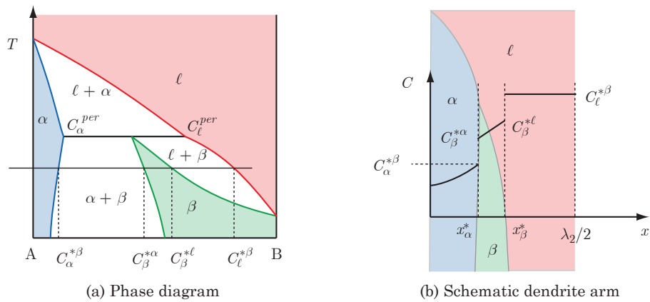
Fig. 10.7 (a) An idealized binary peritectic phase diagram. (b) A schematic drawing of the composition profile behind the dendrite tip where peritectic solidification has begun.
