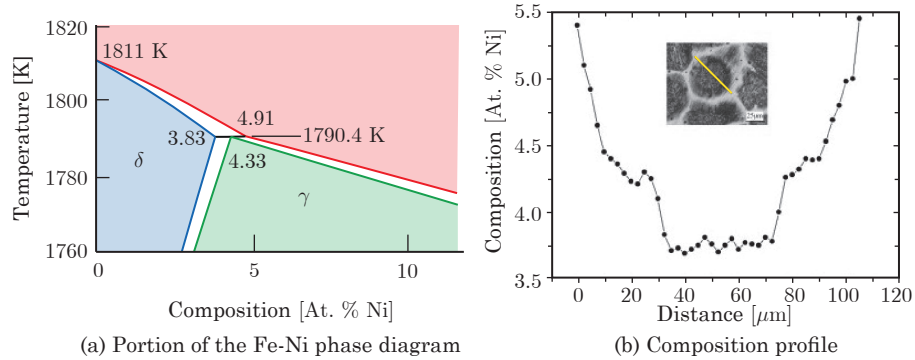
Fig. 10.6 (a) The Fe-rich portion of the Fe-Ni phase diagram. (b) The measured composition profile across a dendrite arm in an alloy of peritectic composition [3]. Copyright 2016 EPFL Press. This figure has been reproduced from Solidification , by J.A. Dantzig and M. Rappaz, for instructional purposes. For other uses, please contact the authors and the EPFL Press for written permission.
