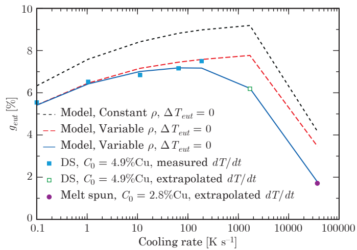
Fig. 10.5 A comparison of results from the microsegregation calculations of Voller and Sundarraj [21] to the experimental data of Sarreal and Abbaschian [11] for Al-Cu alloys.
