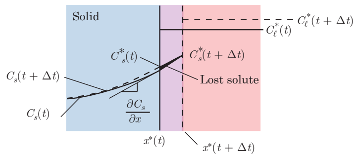
Fig. 10.4 A schematic illustration of the approximation for the solute balance at the interface in the Brody-Flemings model.
