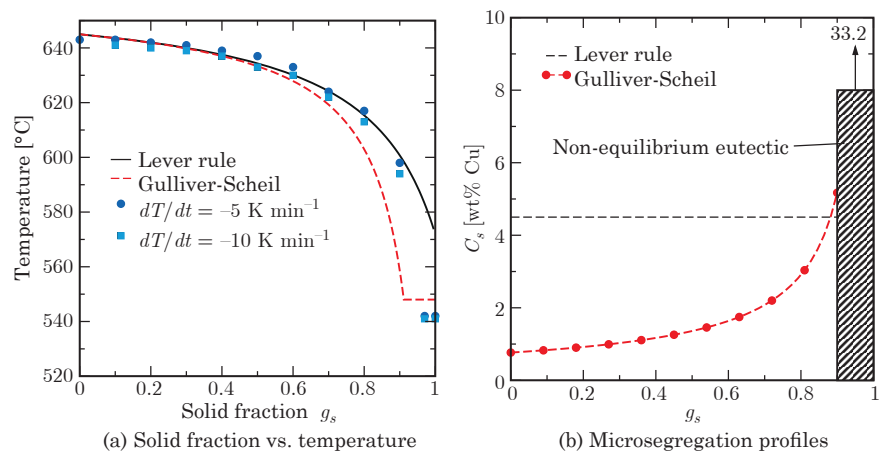
Fig. 10.3 (a) Computed fraction solid vs. temperature curves for an Al-4.5 wt% Cu alloy, using the lever rule and the Gulliver-Scheil equation. The experimental data were obtained by DTA experiments. [8] (b) The corresponding microsegregation patterns for the two solidification models.
