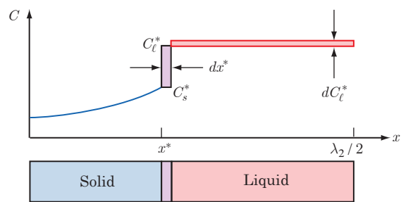
Fig. 10.2 A construct demonstrating the partitioning of liquid from the interface to the liquid in the Gulliver-Scheil model of microsegregation. Copyright 2016 EPFL Press. This figure has been reproduced from Solidification , by J.A. Dantzig and M. Rappaz, for instructional purposes. For other uses, please contact the authors and the EPFL Press for written permission.
