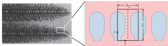
Fig. 10.1 (Left) A micrograph from a directionally solidified succinonitrile-acetone alloy. (Right) An idealized segment, displaying a periodic arrangement of secondary dendrite arms.
