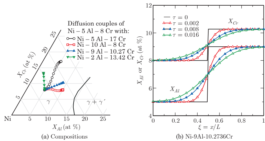
Fig. 10.16 (a) The locus of compositions attained in the various diffusion couples. (b) An alloy along an eigenvector of [D'] . Copyright 2016 EPFL Press. This figure has been reproduced from Solidification , by J.A. Dantzig and M. Rappaz, for instructional purposes. For other uses, please contact the authors and the EPFL Press for written permission.
