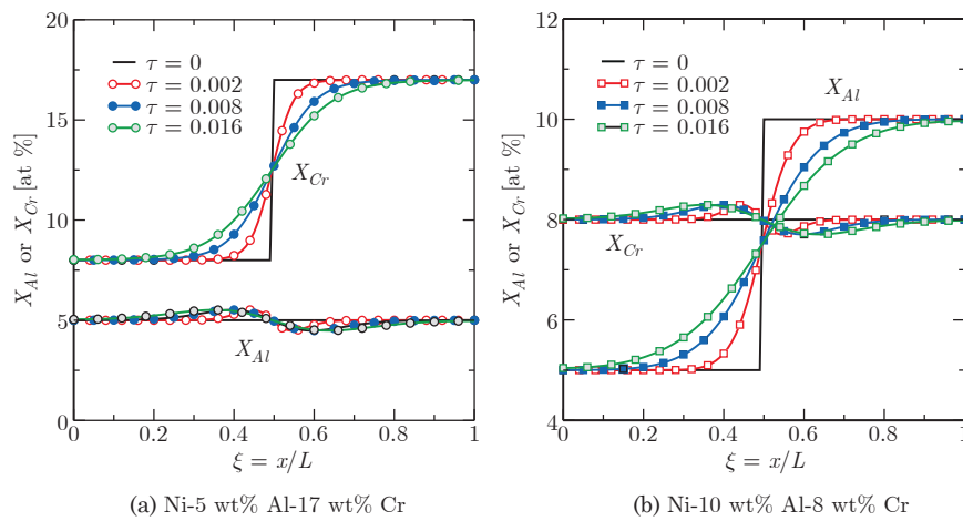
Fig. 10.15 Computed composition profiles in two diffusion couples each with one of the compositions held constant.
