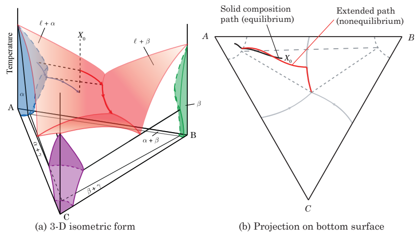
Fig. 10.14 A ternary eutectic equilibrium phase diagram, displaying the solidification path for alloy x in both equilibrium and non-equilibrium solidification. Note that in the latter case, the solid composition is not constrained to pass through the nominal composition.
