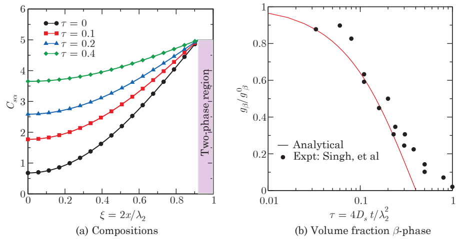
Fig. 10.13 Computed values of (a) compositions in the primary phase and (b) the residual volume fraction \beta -phase for an Al-4Cu alloy.
