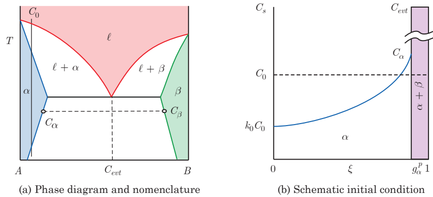
Fig. 10.12 A schematic view of (a) the phase diagram and (b) initial condition for solution treatment analysis.
