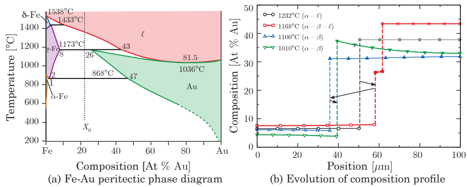
Fig. 10.8 Solidification in the peritectic Fe-Au system. (a) Equilibrium phase diagram. (b) Evolution of the composition profile across a dendrite arm in an alloy of peritectic composition. Filled symbols indicate the liquid phase, filled black symbols the \beta -phase, and open symbols the \alpha -phase. The path from high to low temperatures is indicated by arrows [5].
